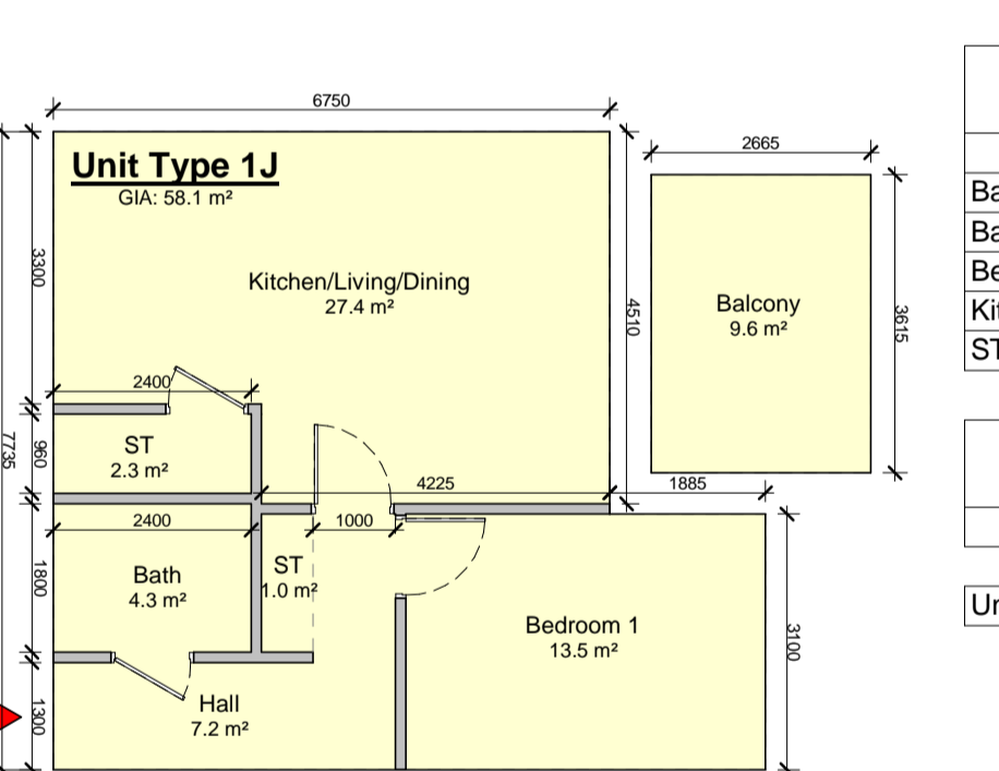
10 Apartment Type 1J 1 : 100
