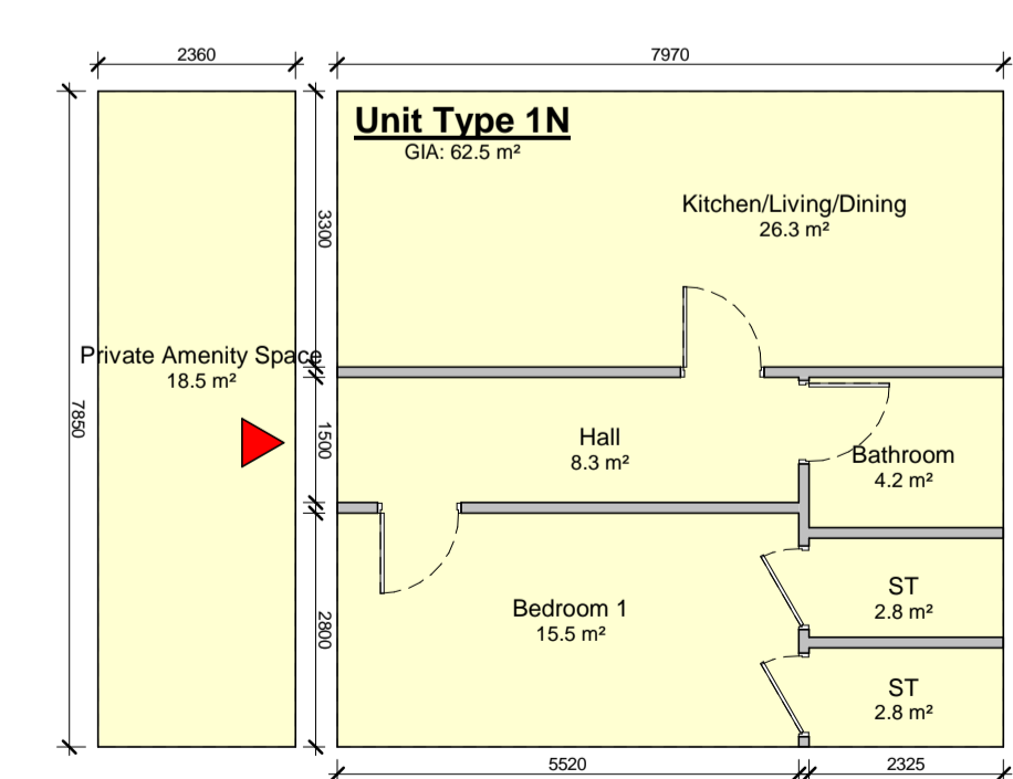
12 Apartment Type 1N 1 : 100
