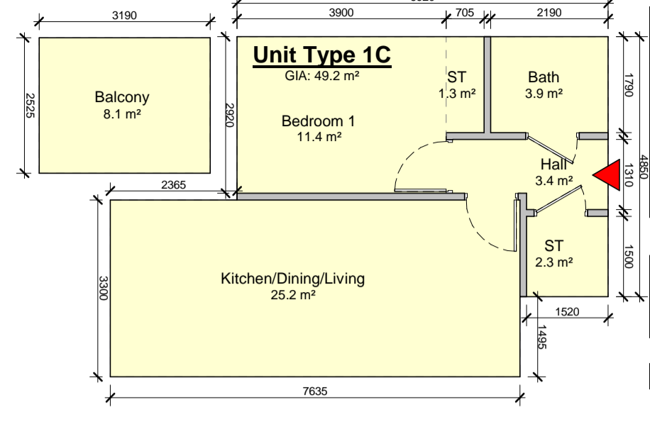
3 Apartment Type 1C 1 : 100
