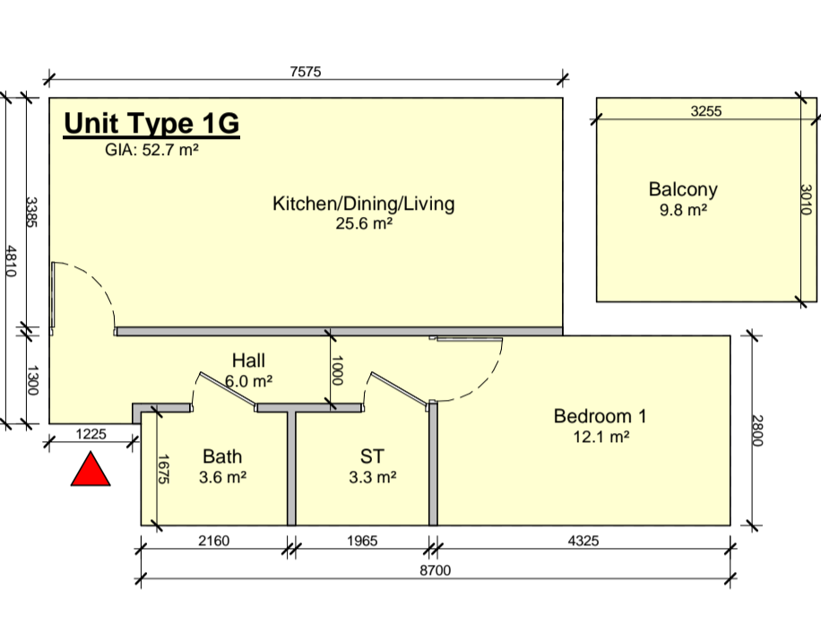
7 Apartment Type 1G 1 : 100
