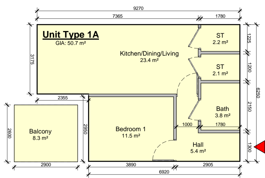
1 Apartment Type 1A 1 : 100
