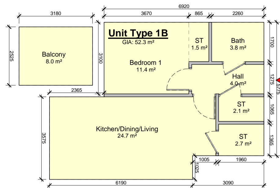
2 Apartment Type 1B 1 : 100
