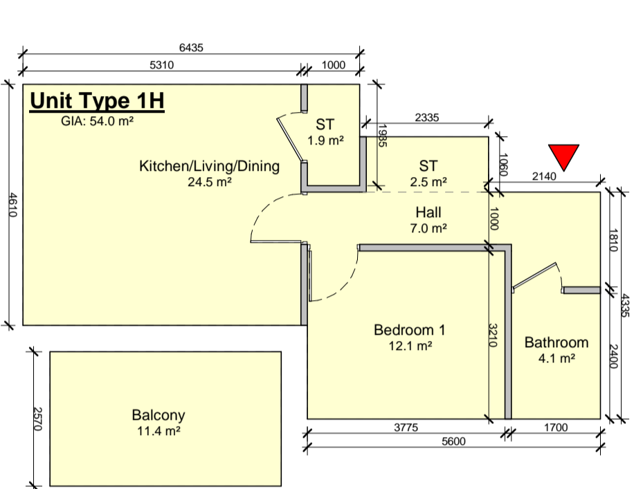
8 Apartment Type 1H 1 : 100
