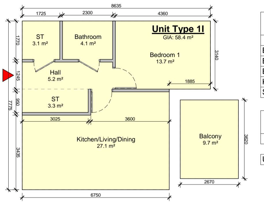
9 Apartment Type 1i 1 : 100
