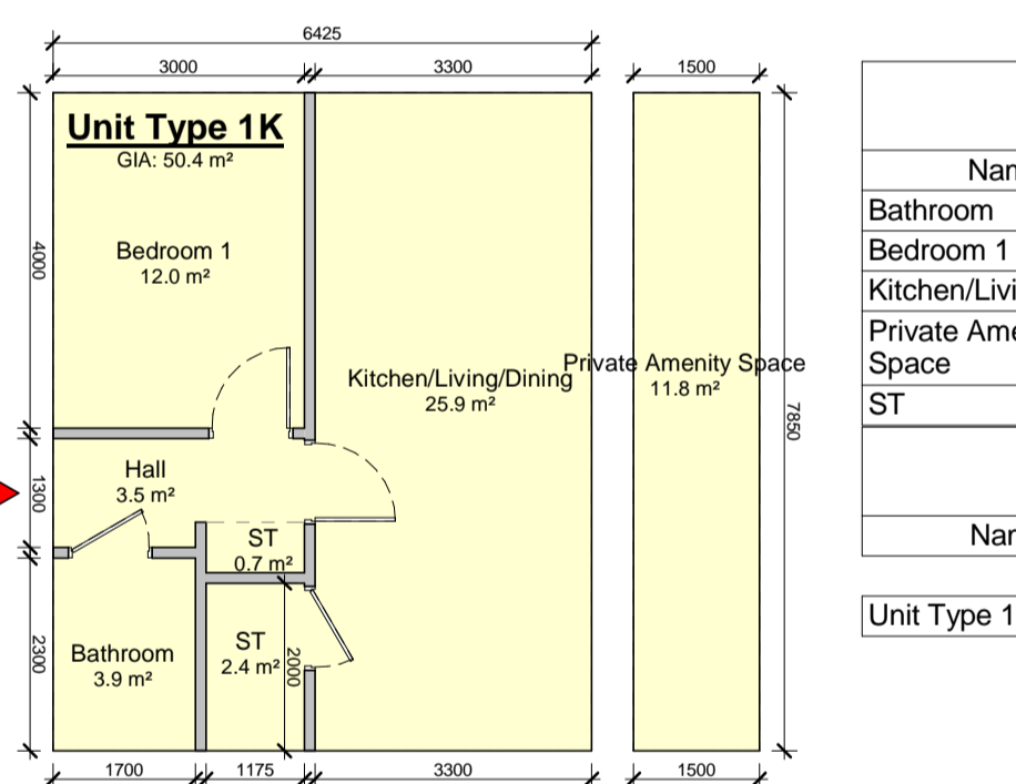
11 Apartment Type 1K 1 : 100
